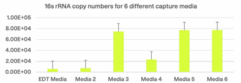
Figure 2. 16S rRNA copy number of five different capture media and EDT media
